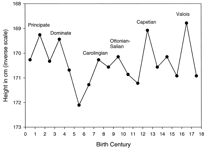
Figure 10.1 Average height of Europeans during the two millennia CE. Data are from skeletal material (Koepeke and Baten 2005). Heights are plotted on an inverse scale, so that the peaks in the graph correspond to population peaks (because periods of high population density should correlate with low average heights).
