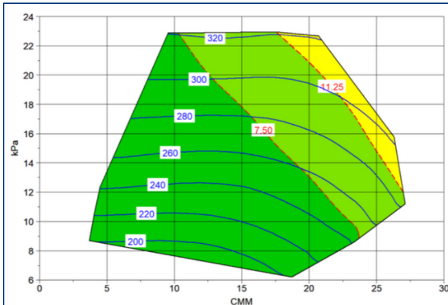
CUSTOM COMPRESSOR MAPS AVAILABLE ON REQUEST
