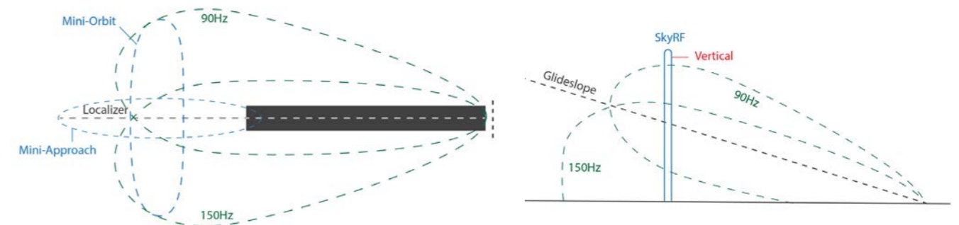
SkyRF trajectories for LLZ and GS measurement of ILS
