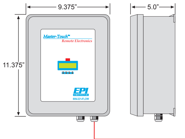
Remote Electronics Enclosure
