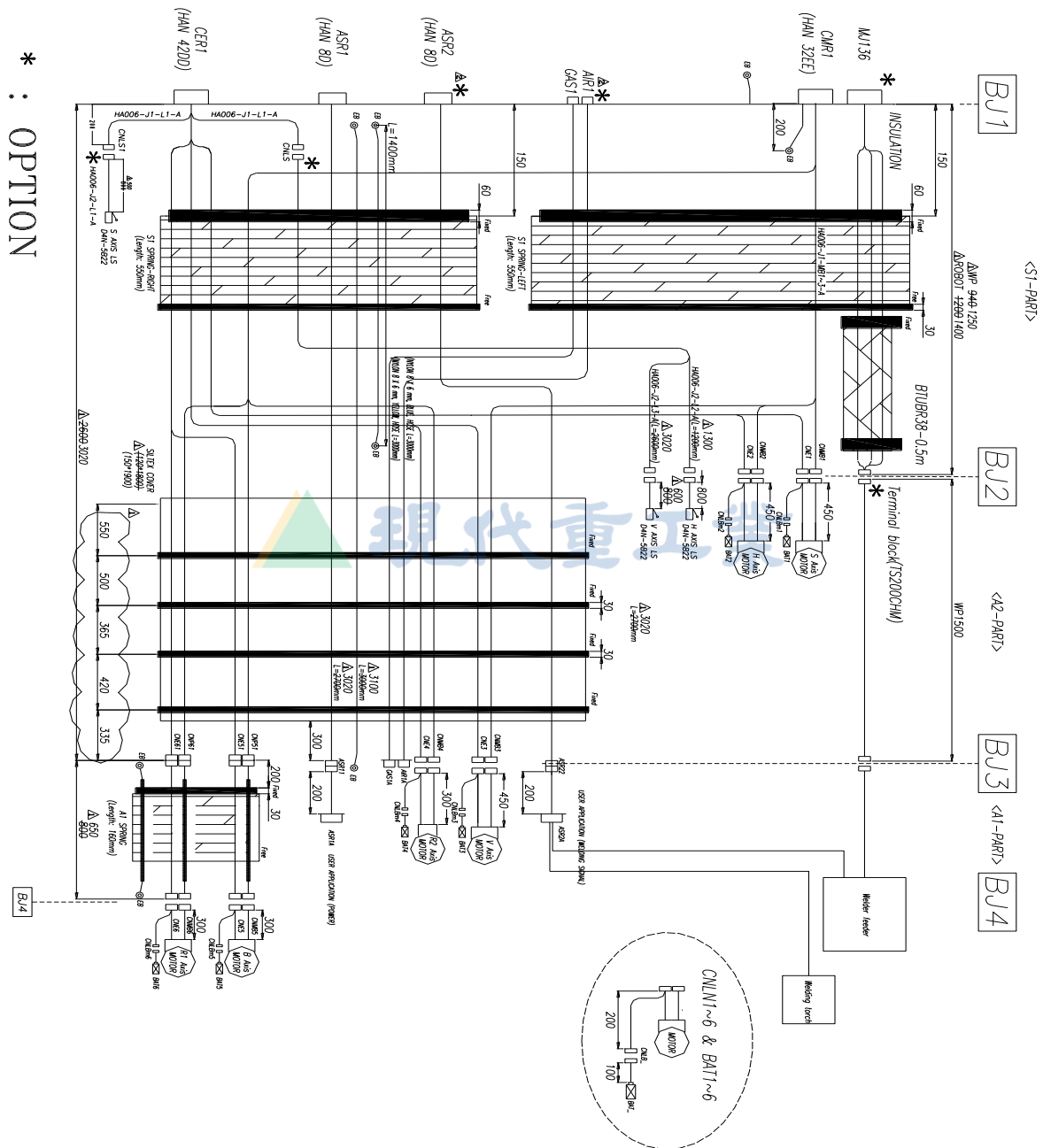
図 8.3 CABLE BLOCK DIAGRAM [HA006A]
