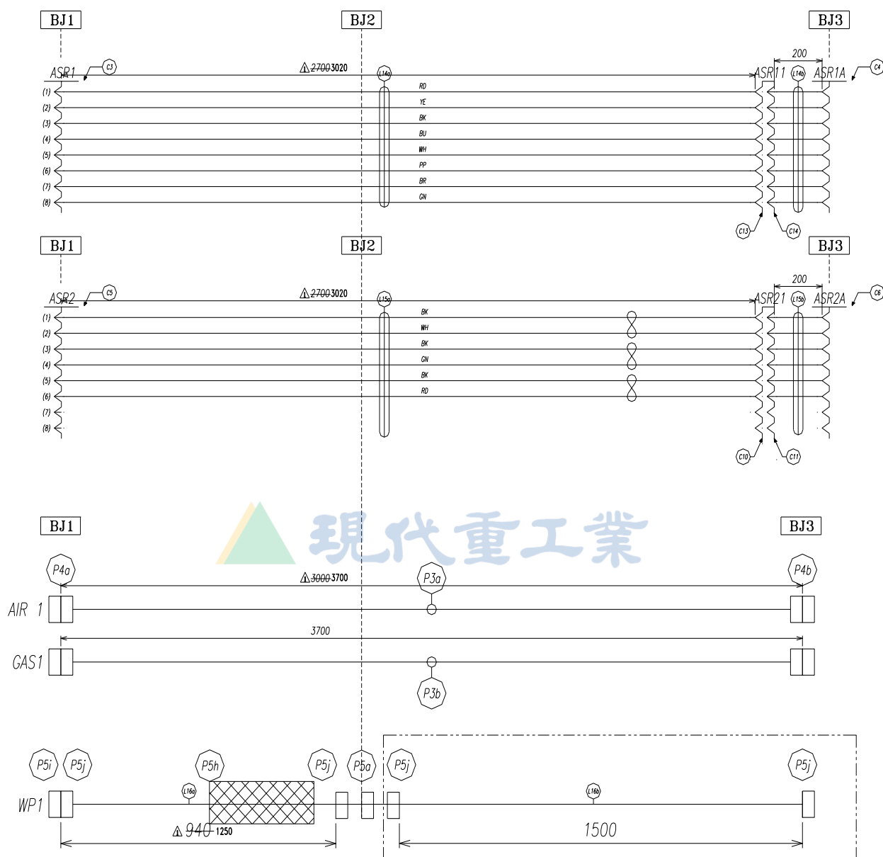
图 8.7 USER APPLICATION &amp; AIR TUBE [HA006A]
