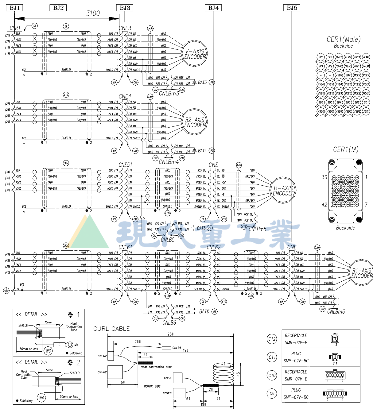
图 8.12 ENCODER CABLE FOR V,R2,B,R1 AXIS [HA020W/HA010LW]
