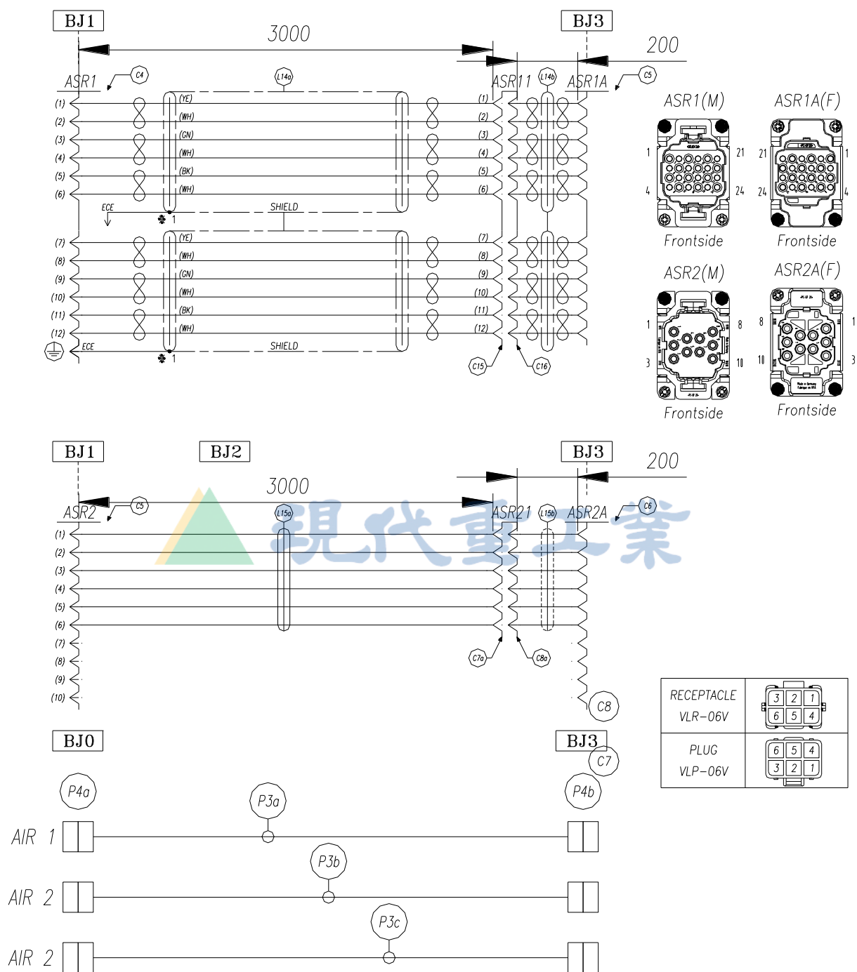
图 8.13 USER APPLICATION &amp; AIR TUBE [HA020W/HA010LW]
