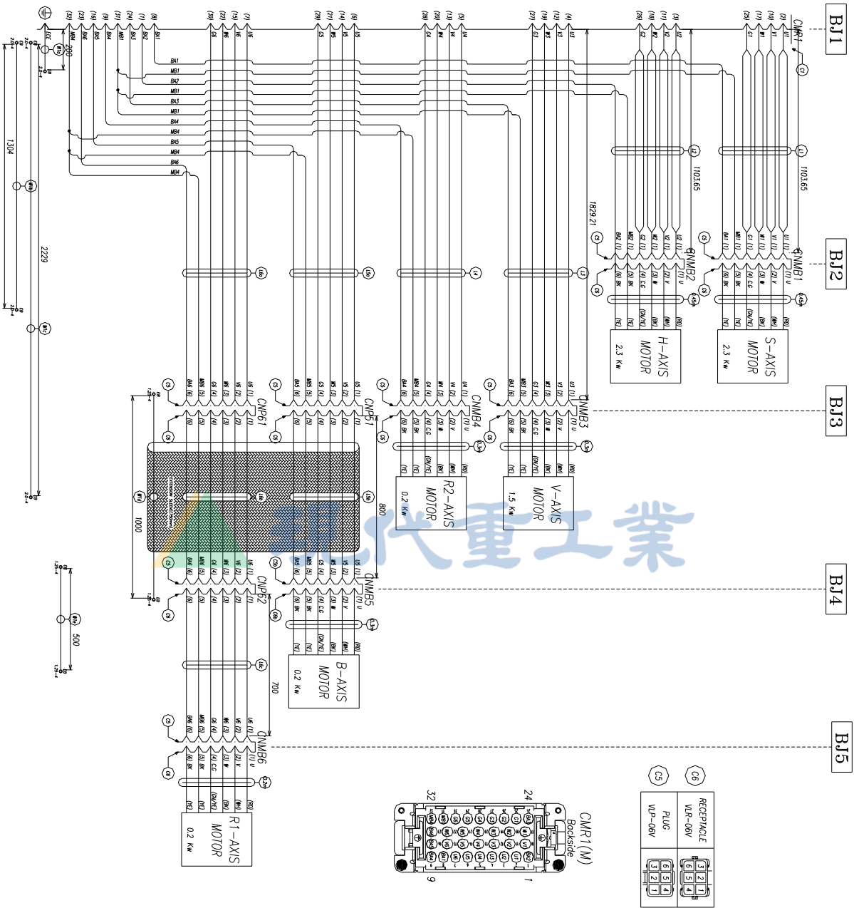
8.4 MOTOR POWER CABLE [HA006]
