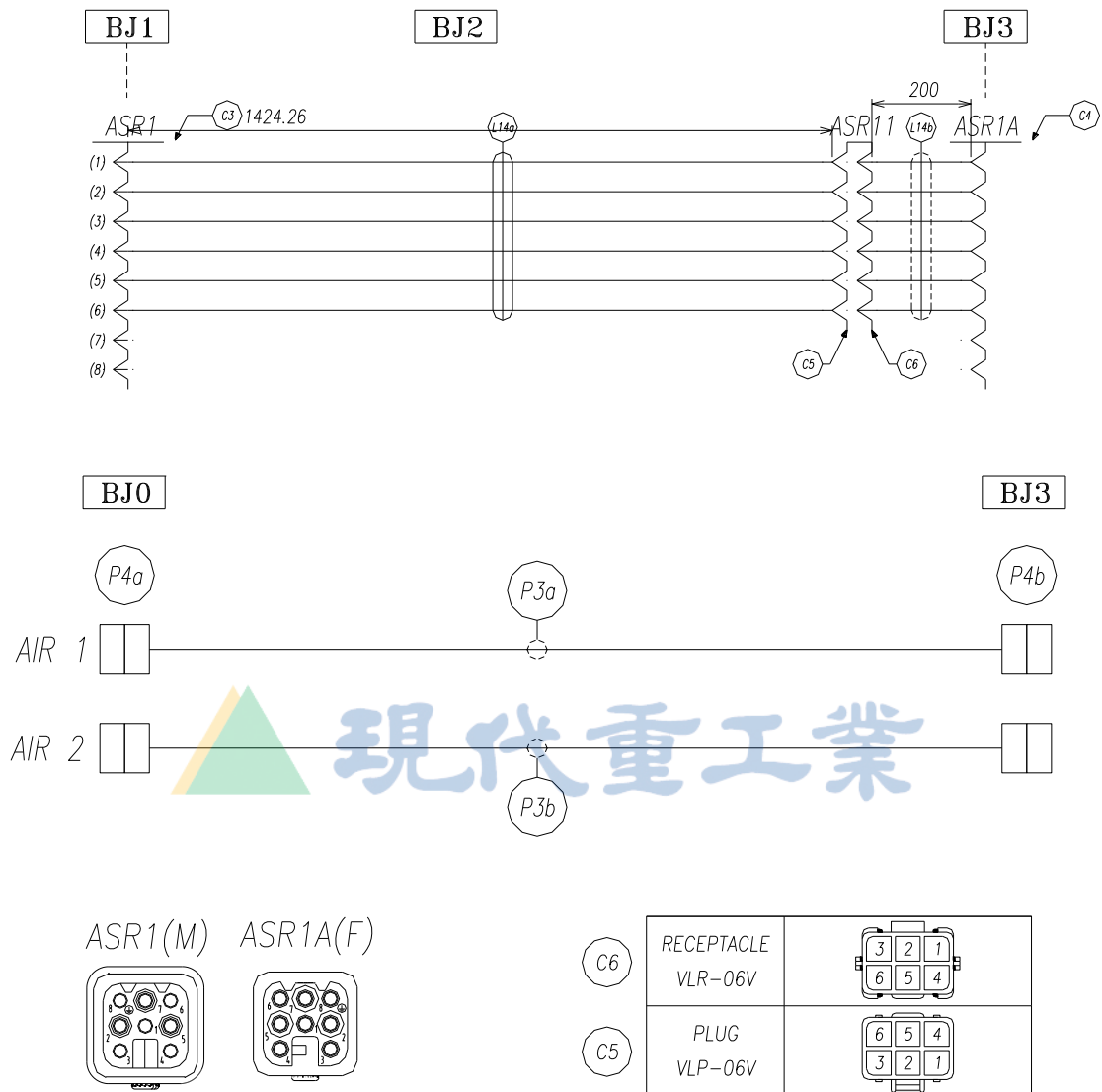
图 8.7 APPLICATION CABLE &amp; AIR TUBE [HA006]
