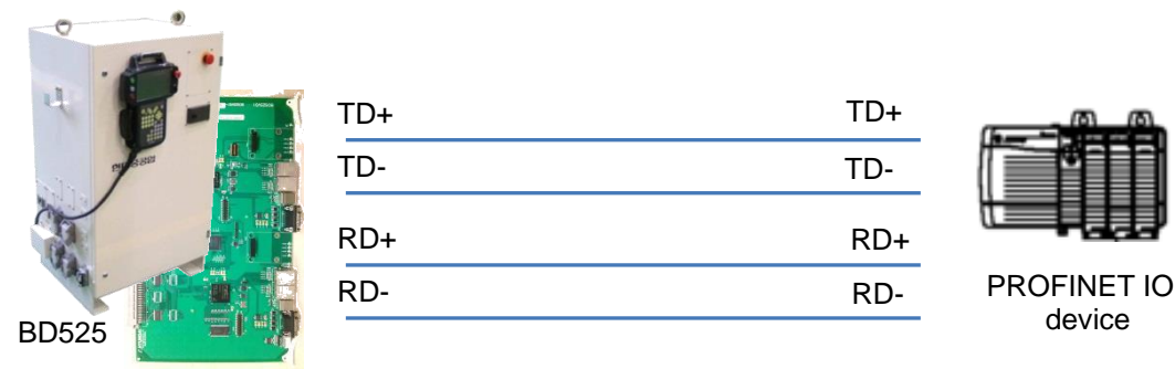
Figure 2.4 Connecting Direct cable
