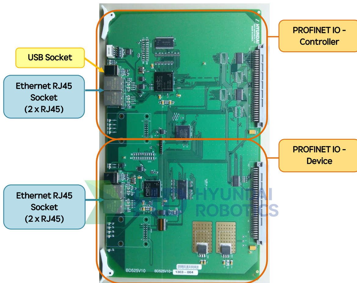
Figure 1.2 BD525 PROFINET IO communication board
