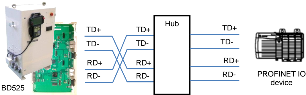
Figure 2.3 Connecting Crossover cable
