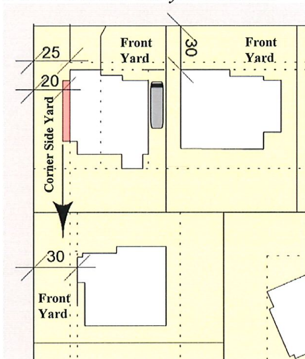
10' building setback differential with a 30' front yard setback
