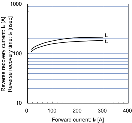
Reverse Recovery Characteristics (typ.) V_{CC}=600\text{V} , V_{GE}=\pm 15\text{V} , R_G=1.1\Omega , T_J=150^{\circ}\text{C}
