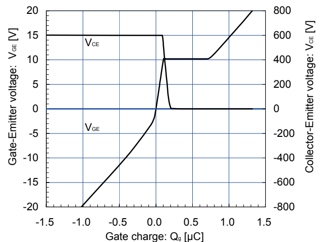
Dynamic Gate Charge (typ.) V_{CC} = 600\text{V} , I_C = 150\text{A} , T_J = 25^\circ\text{C}
