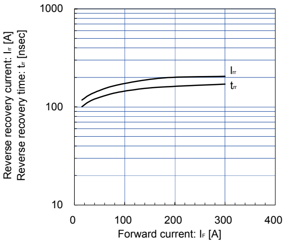
Reverse Recovery Characteristics (typ.) V_{CC}=600\text{V} , V_{GE}=\pm 15\text{V} , R_G=1.1\Omega , T_J=125^{\circ}\text{C}
