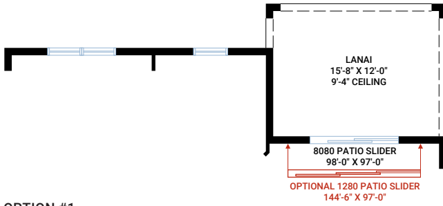
OPTION #1 Extended Covered Lanai - 190 sq ft under roof
