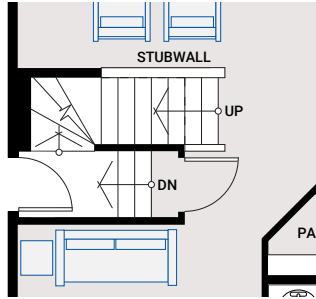
OPTION #05A Exterior Side Entry To Basement - adds 19 sq ft - not available with option 16A
