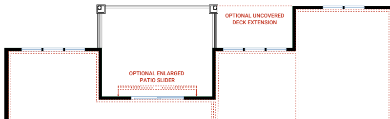
Optional Basement Rear Walk-Out
