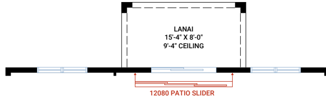
OPTION #1A Covered Lanai - Adds 122 sq ft
