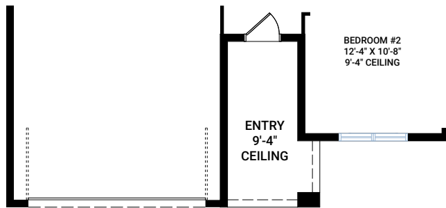
ELEVATION C Craftsman Entry - Entry - 107 sq ft
