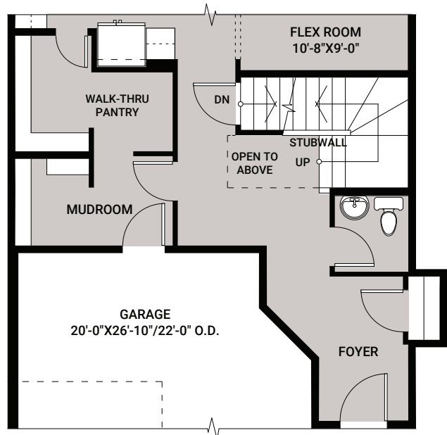
OPTION #02C Walk-thru Pantry / Mudroom - adds 77 sq ft - deletes 77 sq ft from garage
