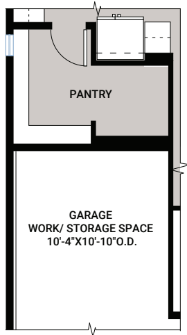
OPTION #02A Enlarged Pantry - adds 43 sq ft - deletes 43 sq ft from garage
