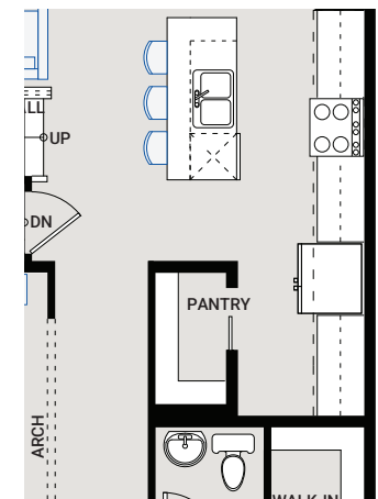
OPTION #02C Alternate Kitchen - no additional sq ft - additional kitchen cabinetry added - revised pantry layout
