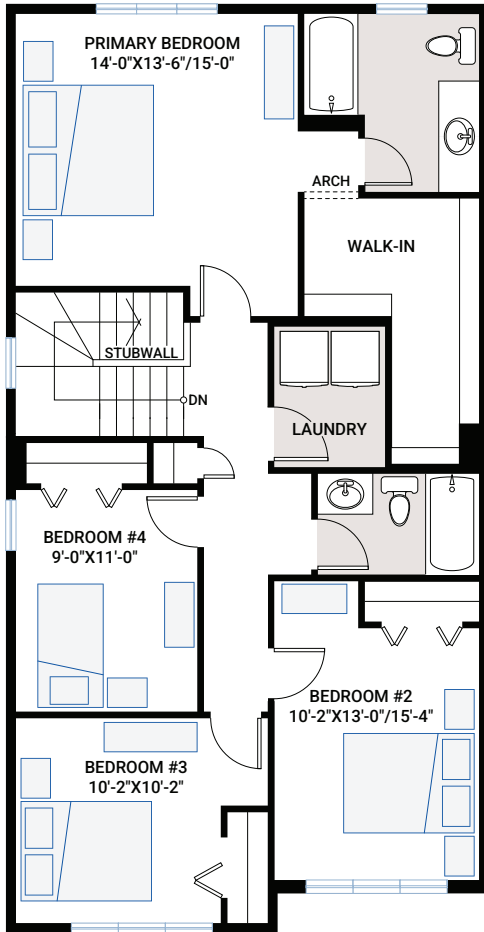
OPTION #04A Alternate Upper Floor 4th Bedroom - no additional sq ft - replace loft with 4th bedroom
