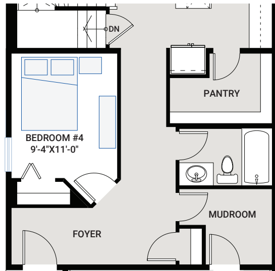
OPTION #03B Main Floor Bedroom And Bathroom - no additional sq ft
