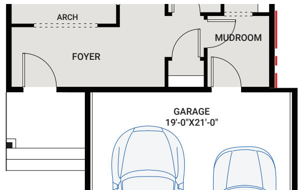
OPTION #05B 2'-0" Garage Shift - no additional sq ft - porch becomes 7 feet wide
