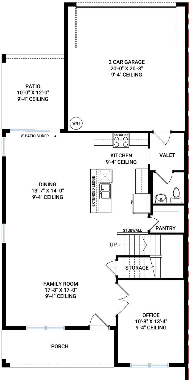
MAIN FLOOR
