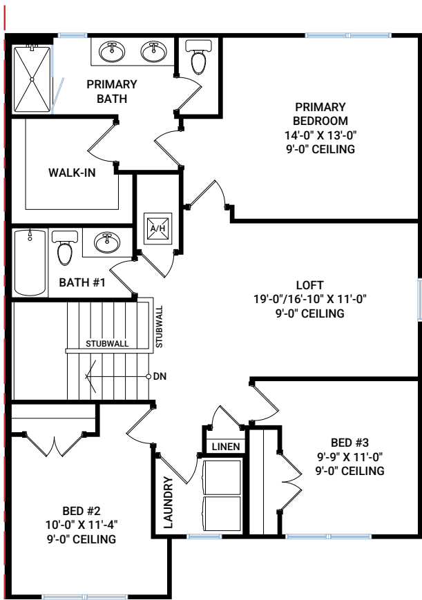
UPPER FLOOR
