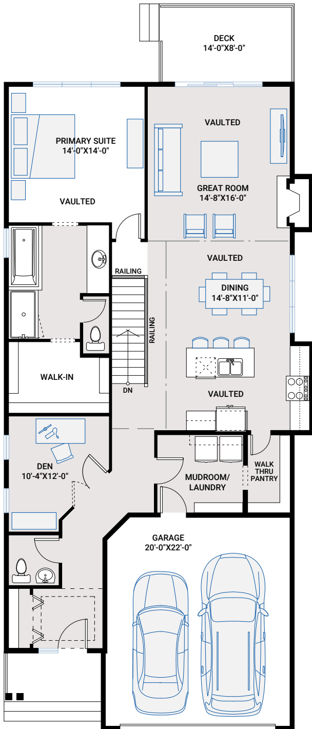
OPTION #20A Vaulted Ceiling - does not include window upgrades
