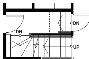
Partial Main Floor Plan
