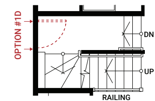
Partial Main Floor Plan
