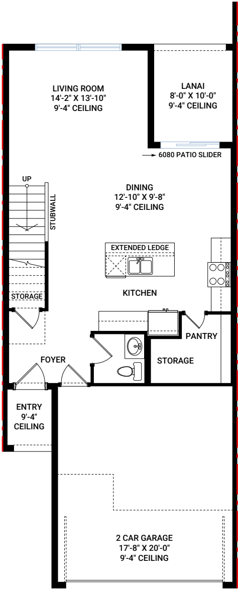
MAIN FLOOR
