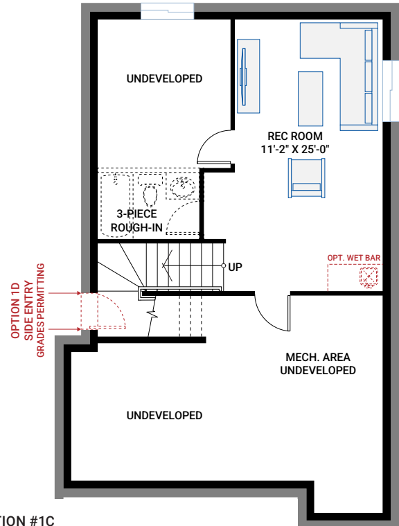
OPTION #1C Developed Basement Rec Room - additional 304 sq ft - Includes Option #1A - Developed Basement Stairs
