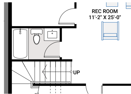
OPTION #1F Developed Basement Bathroom - only available with Option #1C - adds 48 sq ft to Developed Basement
