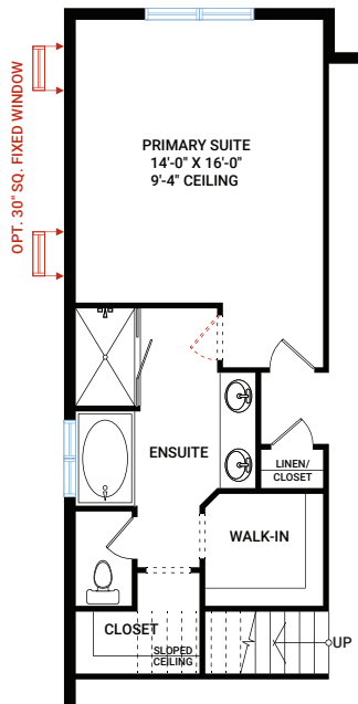
OPTION #3 WITH OPTION #4 COMBINED Alternate Primary Suite Bathroom With Tub - adds 38 sq ft to main floor living space
