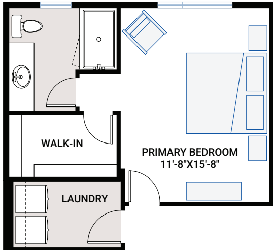
OPTION #01A Alternate Ensuite - adds 44 sq ft - cantilever rear 2'-0" - remove flush beam over nook. Main floor cantilever to carry second floor roof load.
