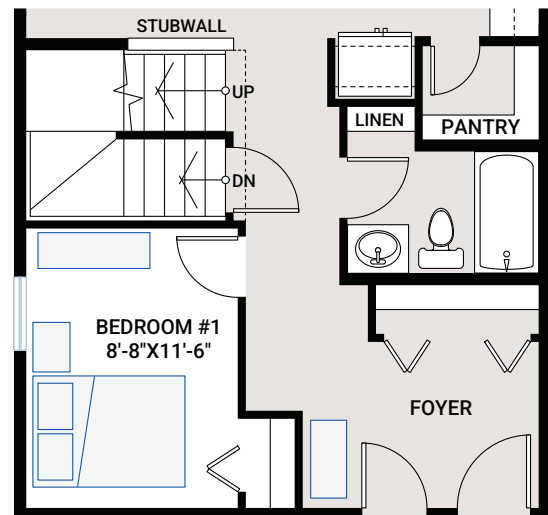
OPTION #03B Main Floor Bedroom/Bathroom - no additional sq ft
