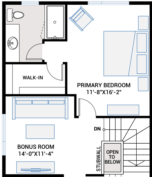
OPTION #01A Alternate Ensuite - adds 44 sq ft - cantilever rear 2'-0"
