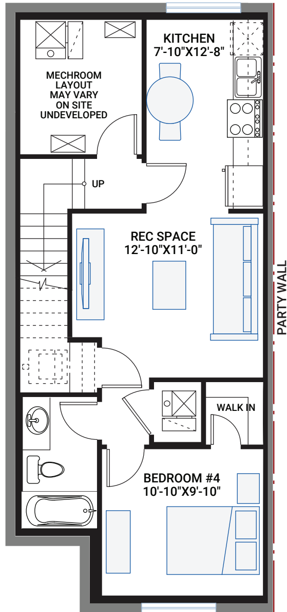
CONCEPTUAL BASEMENT SUITE - adds 571 sq ft
