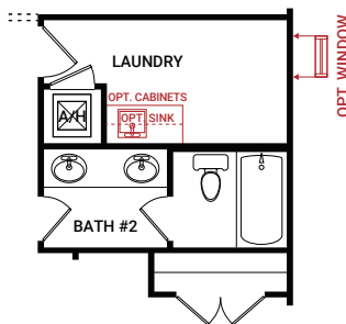
OPTION #2 Jack and Jill Bathroom Replaces Standard Bathroom
