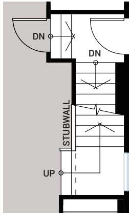
OPTION #05A Exterior Side Entry to Basement
