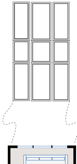
OPTION #05A Alternate Two-Storey Family Room Window - revised window configuration
