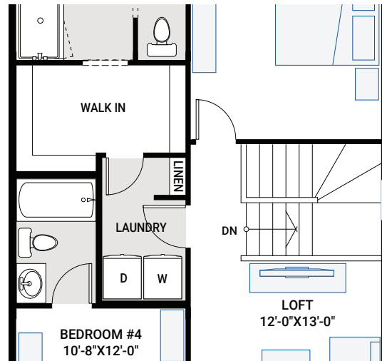
OPTION #05D Walk-Thru Laundry Room - no additional sq ft
