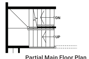
OPTION #4A 9'-0" Basement Ceiling - adds two risers to Basement stairs, consisting of one winder on lowest landing and one tread on bottom run.
