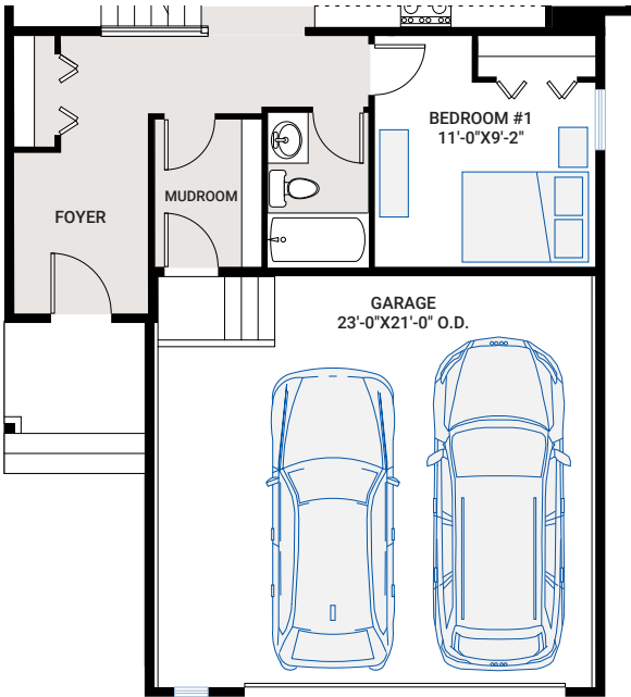
OPTION #01B Alternate Main Floor - adds 34 sq ft - full bath added to Main Floor - Flex Room revised to Main Floor bedroom
