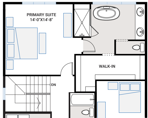
OPTION #10B Alternate Primary Ensuite - adds 45 sq ft
