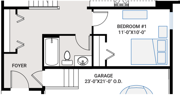
OPTION #01A Alternate Main Floor - no additional sq ft - full bath added to Main floor - Flex Room revised to be Main Floor bedroom
