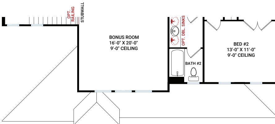
Elevation B Upper
