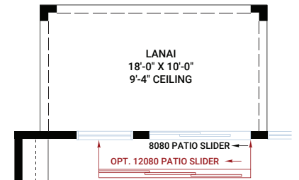
Covered Lanai - adds 180 sq ft under roof
