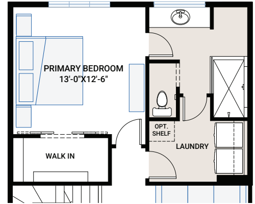
OPTION #10D Alternate Primary Bath - no additional sq ft
