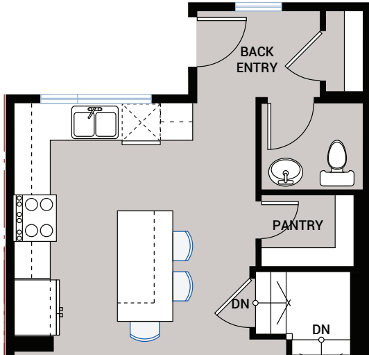
OPTION #03A Rear Entry - adds 70 sq ft
