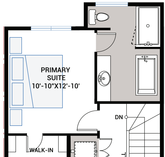
OPTION #01A Alternate Primary Bath - adds 30 sq ft - only available with option 03A or 03B
