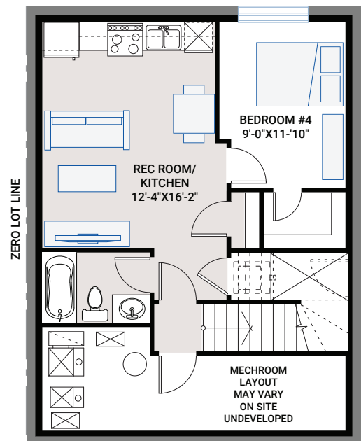
OPTION #100A Basement Secondary Suite Concept
