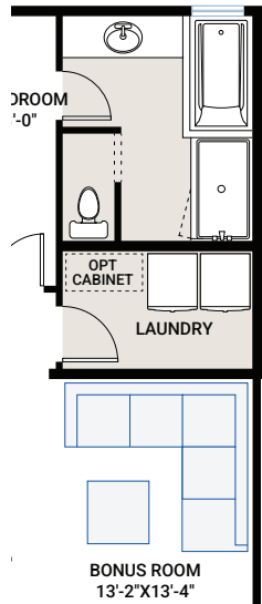
OPTION #10B Alternate Primary Bath - adds 24 sq ft
