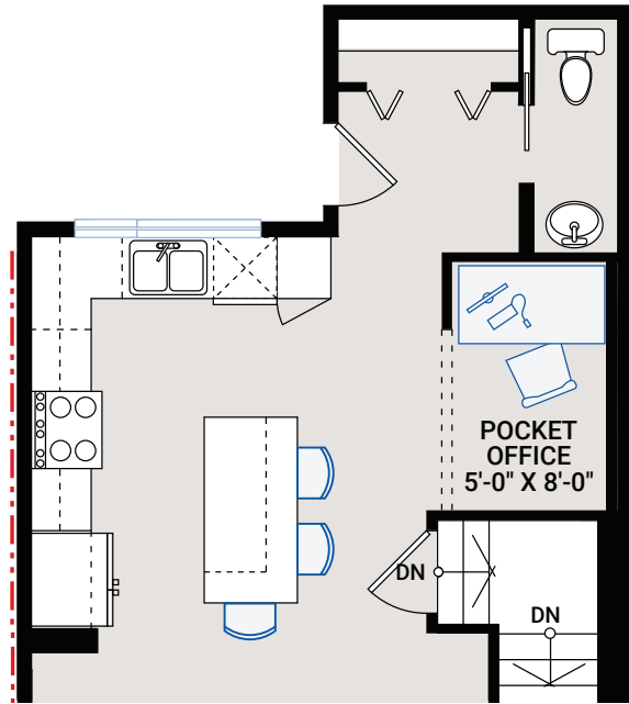
OPTION #03B Rear Entry - adds 90 sq ft
