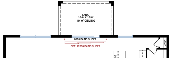
Extended Lanai - adds 160 sq ft under roof
