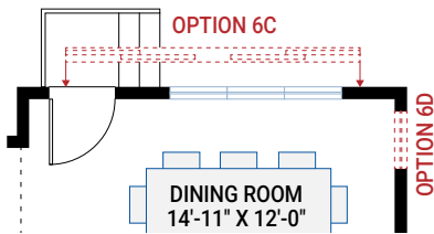
Partial Main Floor Plan
