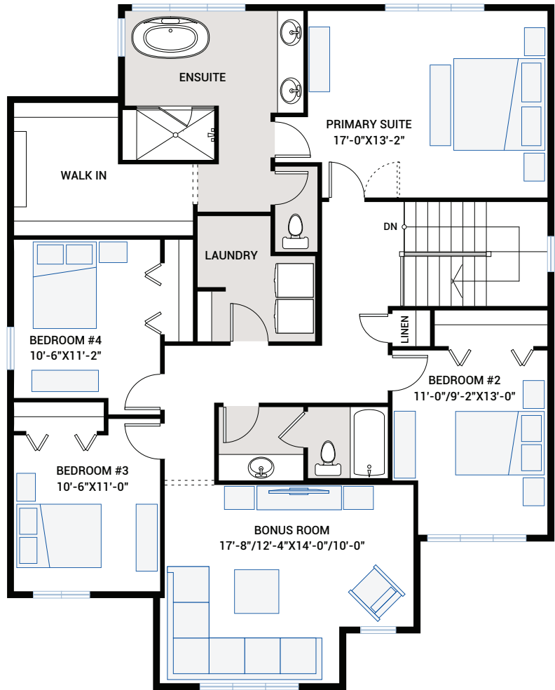
OPTION #04B Alternate Upper Floor - adds 278 sq ft to upper floor
