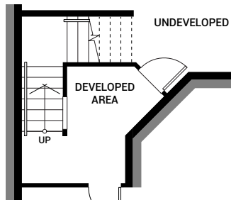
Partial Basement Plan
