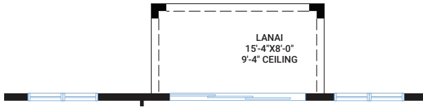
OPTION #1 Covered Lanai - 12' patio slider - 122 sq ft under roof
