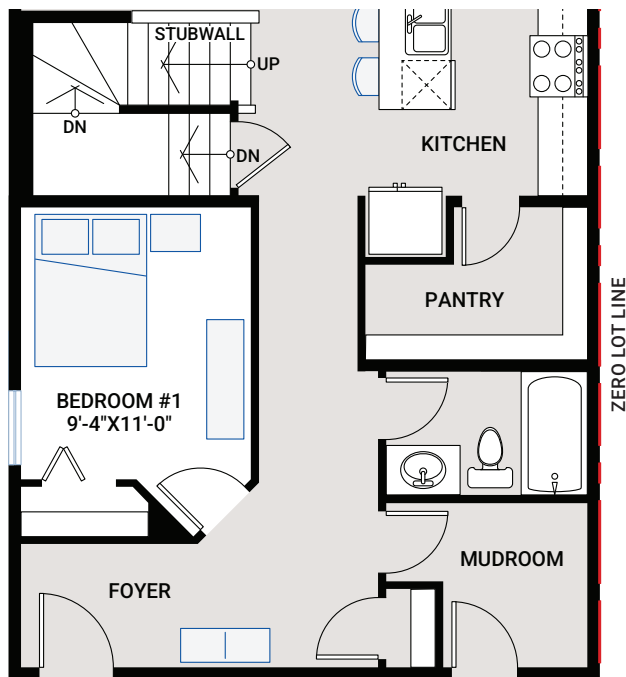
OPTION #03B Main Floor Bedroom and Bathroom - no additional sq ft
