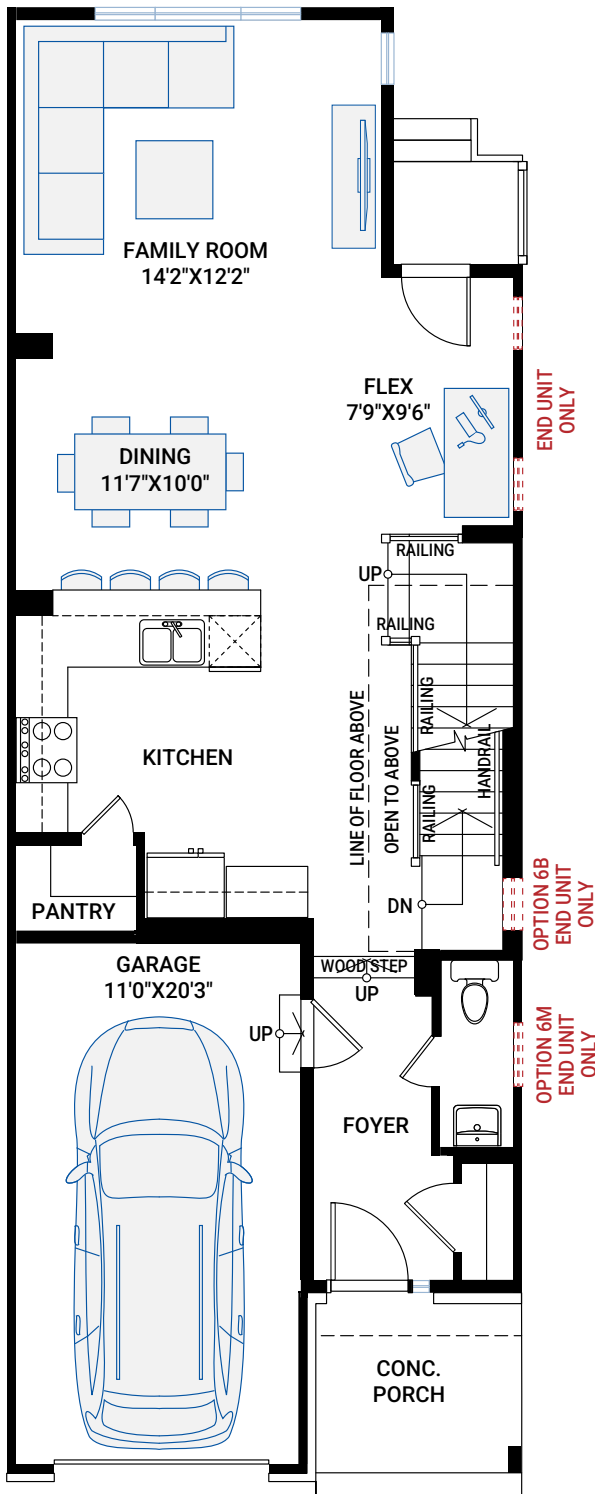
Option #2M Alternate Main Floor
