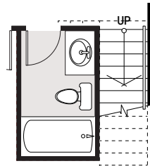
OPTION #1F Basement 3-Piece Bathroom
