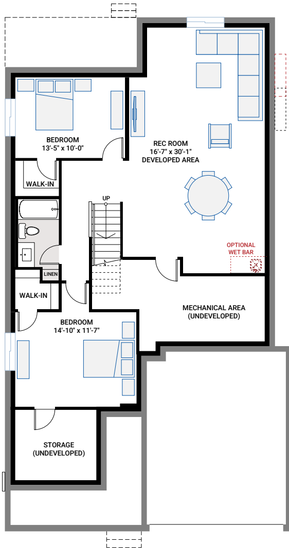
OPTION #1B Developed Basement - Additional basement window in front bedroom - Adds 1,137 sq ft of developed basement
