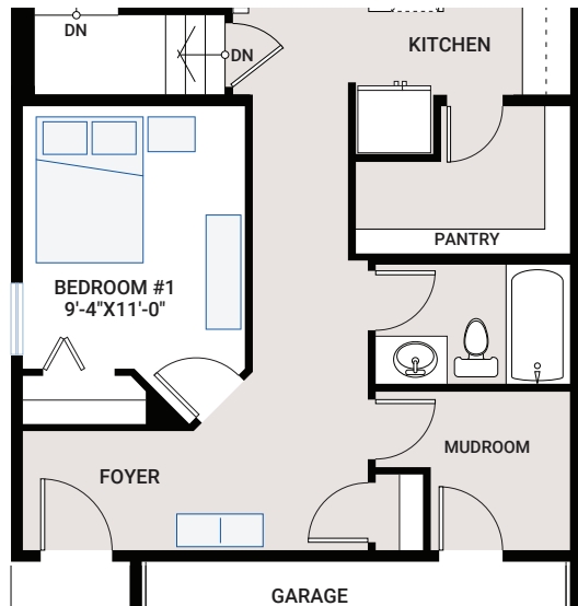
OPTION #03B Main Floor Bedroom and Bathroom - no additional sq ft
