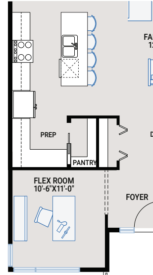
OPTION #02A Prep Kitchen - no additional sq ft - cabinets extended - smaller pantry and larger island
