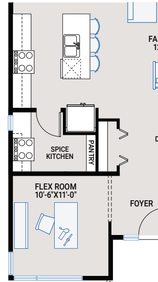
OPTION #02B Spice Kitchen - no additional sq ft - range with cabinets added
