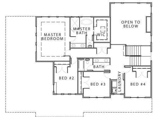
UPPER FLOOR
